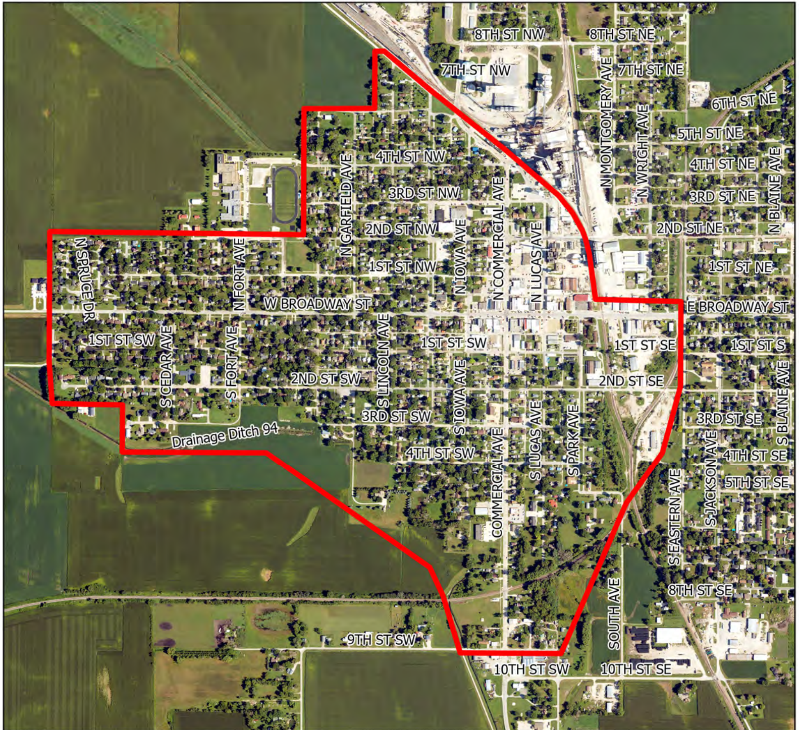
City of Eagle Grove 2025 Sanitary Sewer Collection System Improvement Project Eagle Grove, IA (Wright County)
